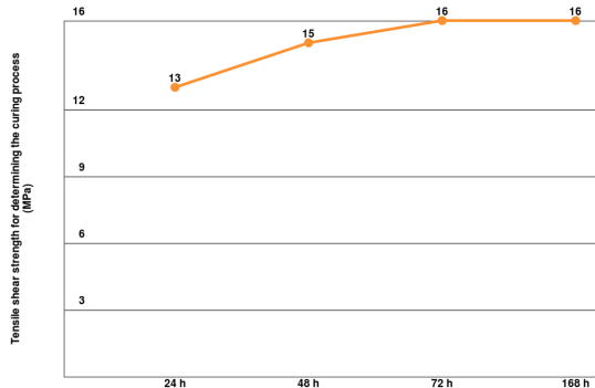
Substrates: Al/Al, based on DIN EN 1465
