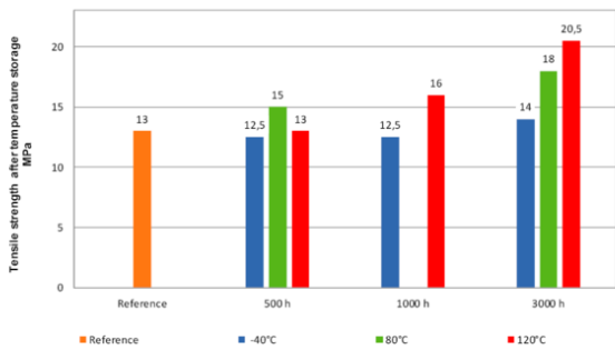
Tensile strength after temperature storage / based on DIN EN ISO 527
