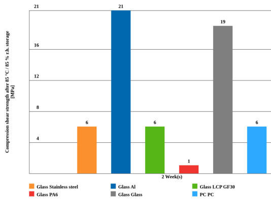
Compression shear strength after 85 °C / 85 % r.h. storage, based on DELO-Norm 5
