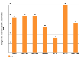
Compression strength after postcuring based on DELO-Norm 5
